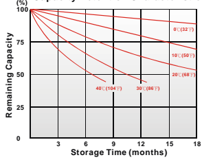
Capacity Retention Characteristic
