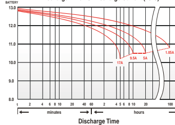
Discharge Time VS. Discharge Current (25°C)
