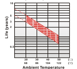
Trickle (or float) Service Life
